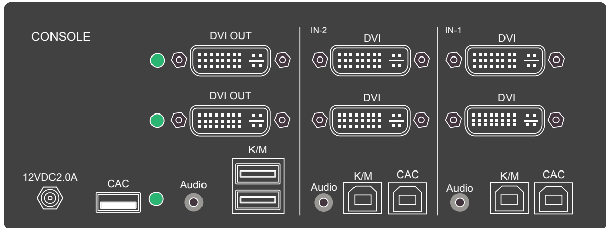
SDPN-2D-P Back
